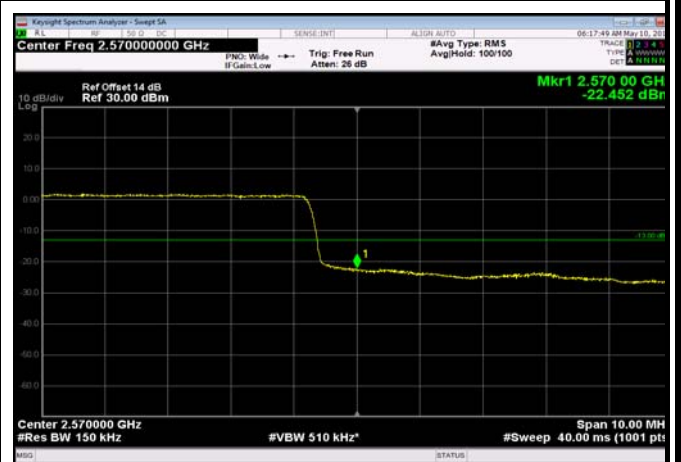
HighRange_FDD07_15MHz_2562.5_fullRB _High_QPSK
