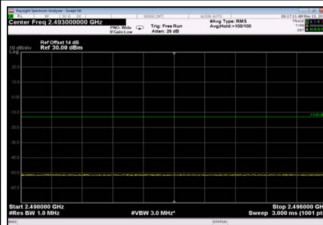
FDD07_15MHz_2562.5_QPSK_OneRB_low _ExtraBands_Range_2490~2496
