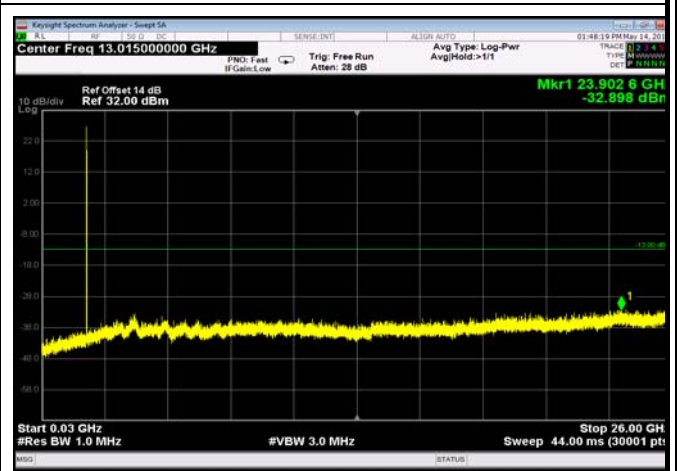
FDD04_HighRange_1.4MHz_30MHz~26GHz
