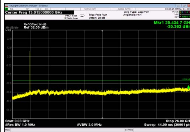
FDD07_HighRange_20MHz_30MHz~26GHz
