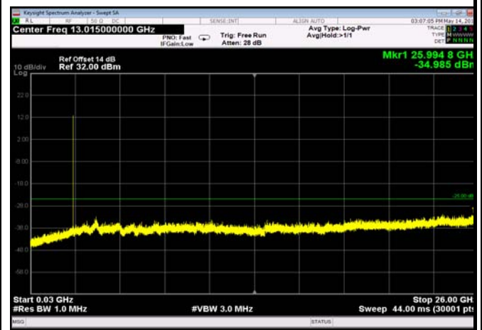
FDD07_MidRange_15MHz_30MHz~26GHz
