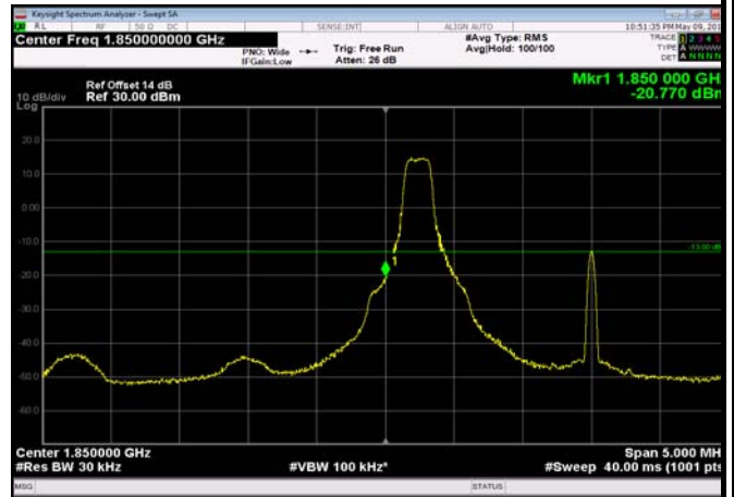
LowRange_FDD02_3MHz_1851.5_fullIRB_low_Q16 16
