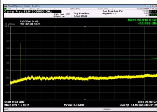
FDD02_MidRange_5MHz_30MHz~26GHz
