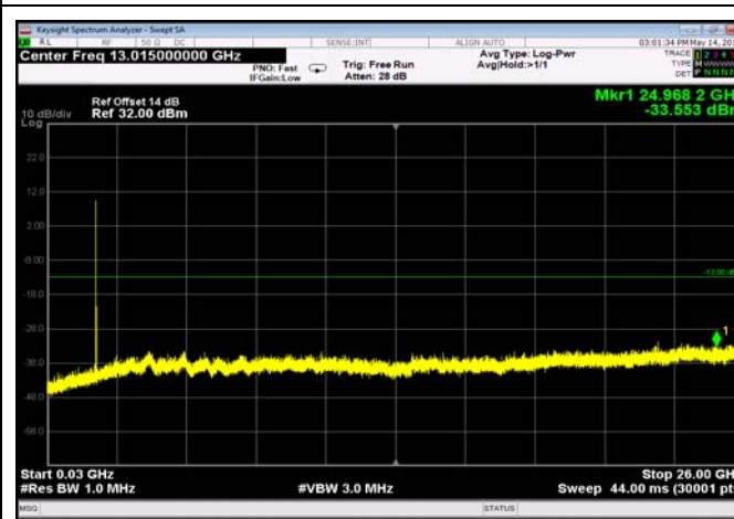
FDD02_LowRange_5MHz_30MHz~26GHz
