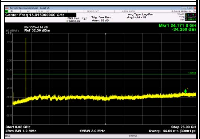
FDD02_MidRange_1.4MHz_30MHz~26GHz
