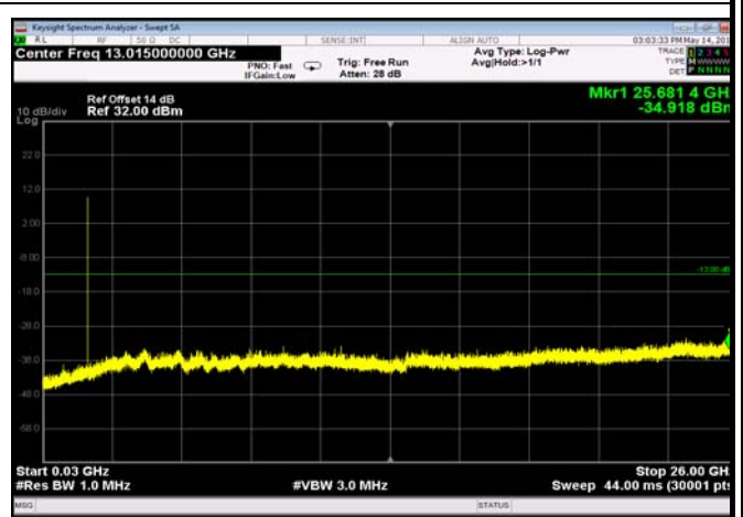
FDD04_MidRange_15MHz_30MHz~26GHz
