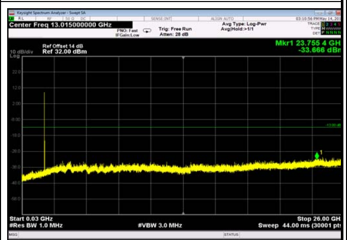
FDD02_LowRange_20MHz_30MHz~26GHz
