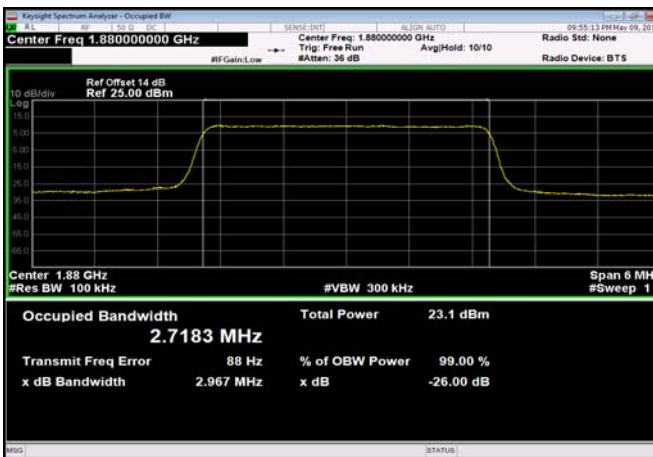
FDD02_MidRange_5MHz_1880MHz_QPSK
