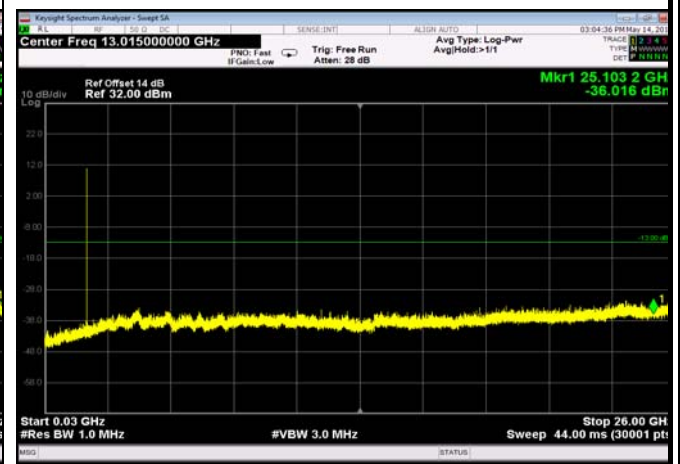
FDD04_LowRange_15MHz_30MHz~26GHz
