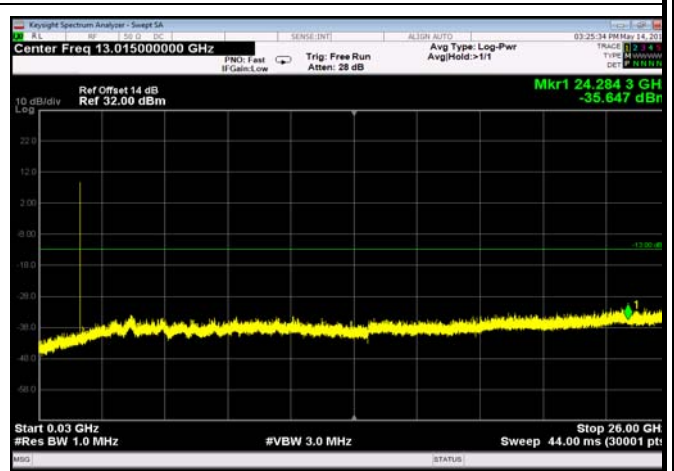
FDD04_MidRange_5MHz_30MHz~26GHz
