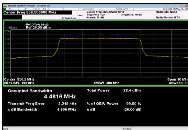
FDD05_MidRange_5_836.5_Q16
