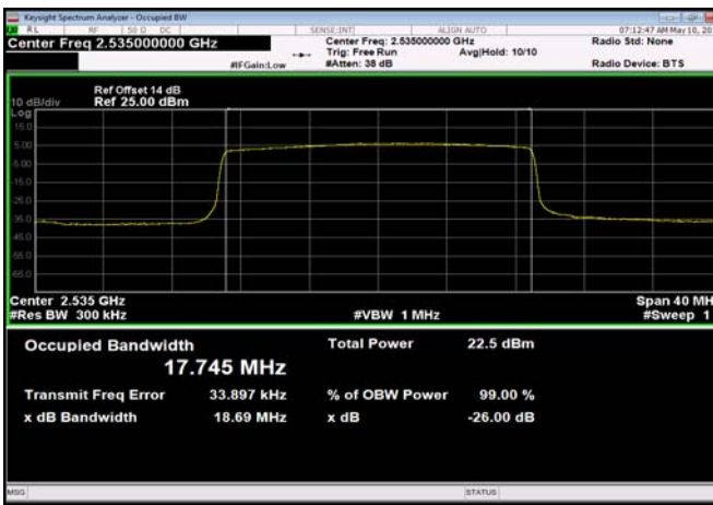
FDD07_MidRange_20_2535_QPSK
