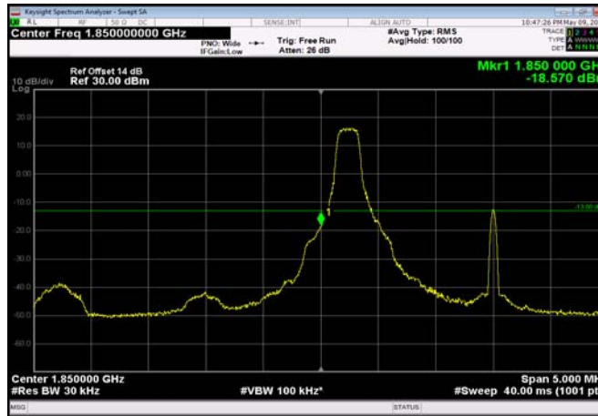
LowRange_FDD02_3MHz_1851.5_fullIRB_low_QPSK 15
