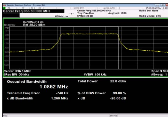
FDD05_MidRange_3_836.5_Q16
