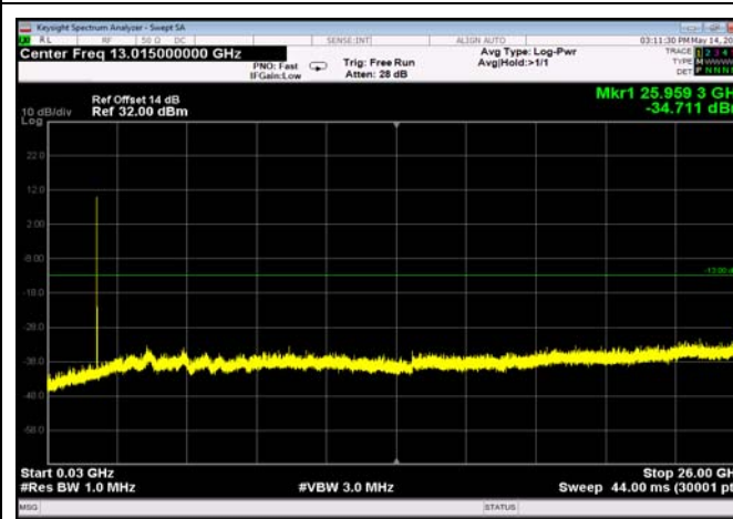
FDD02_MidRange_20MHz_30MHz~26GHz
