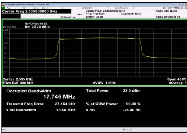
FDD07_MidRange_20MHz_2535MHz_QPSK
