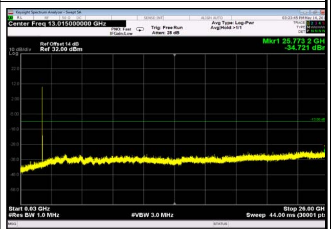
FDD02_MidRange_3MHz_30MHz~26GHz
