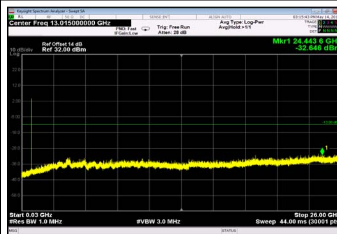
FDD07_HighRange_10MHz_30MHz~26GHz
