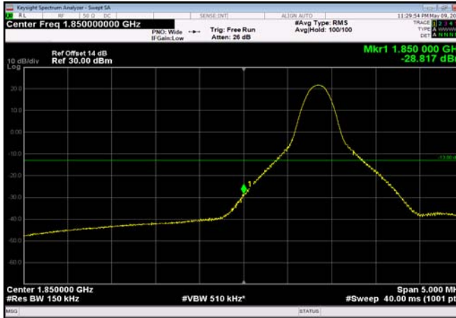
LowRange_FDD02_15MHz_1857.5_fullIRB _Low_QPSK
