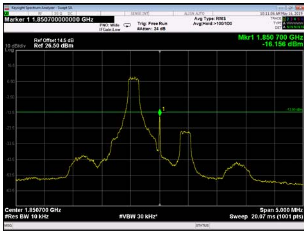
LowRange_FDD02_1.4MHz_1850.7_fullRB _Low_QPSK
