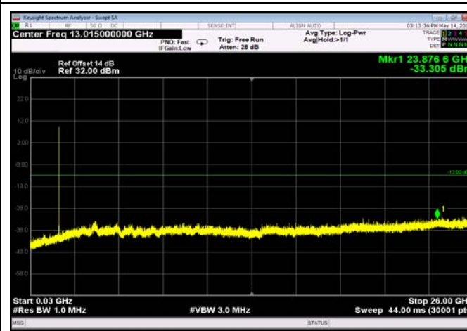
FDD04_MidRange_20MHz_30MHz~26GHz
