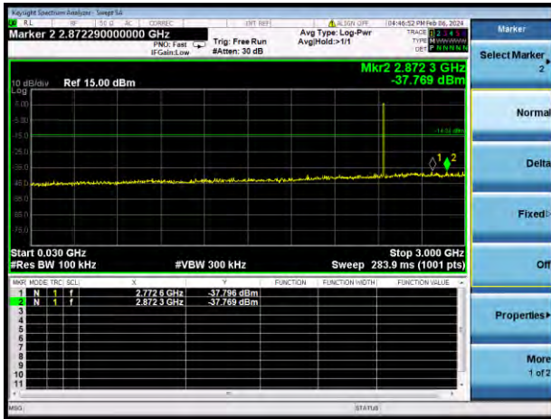
GFSK (BLE 1Mbps) MIDDLE CHANNEL, SPURIOUS 30 MHz ~ 3 GHz
