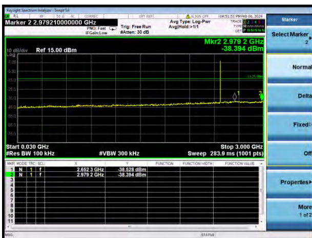
GFSK (BLE 1Mbps) HIGH CHANNEL, SPURIOUS 30 MHz ~ 3 GHz
