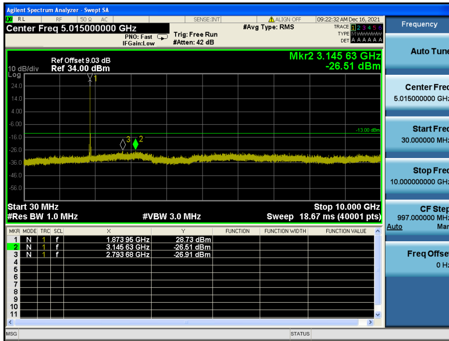
LTE Band 25(2) / 20 MHz / 16QAM - RB Size/Offset (1/0)–Mid Channel
