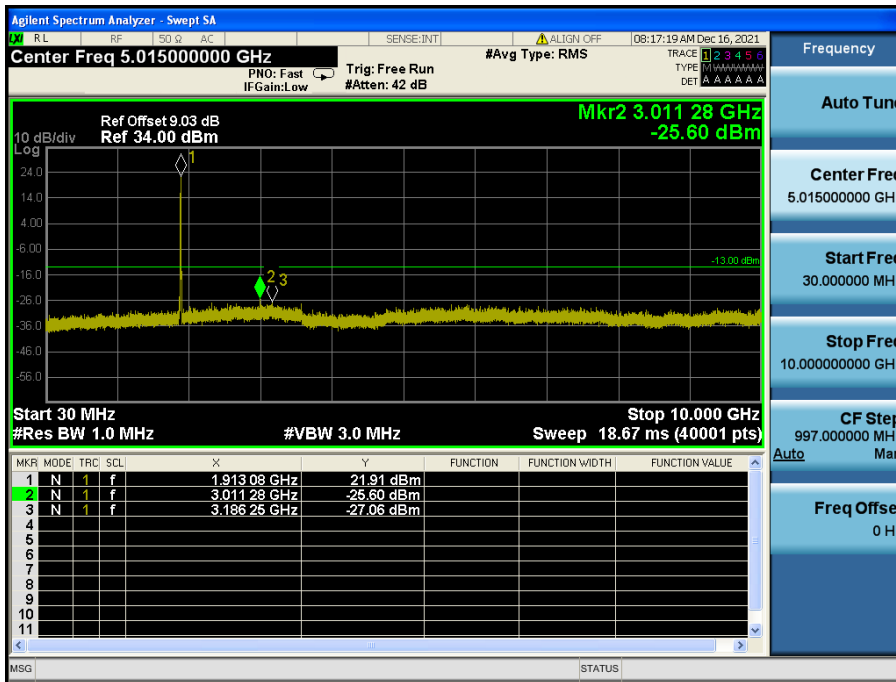
LTE Band 25(2) / 10 MHz / 16QAM - RB Size/Offset (50/0) – High Channel
