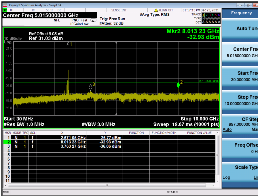
LTE Band 41 / 20 MHz / QPSK - RB Size/Offset (1/0) – High Channel
