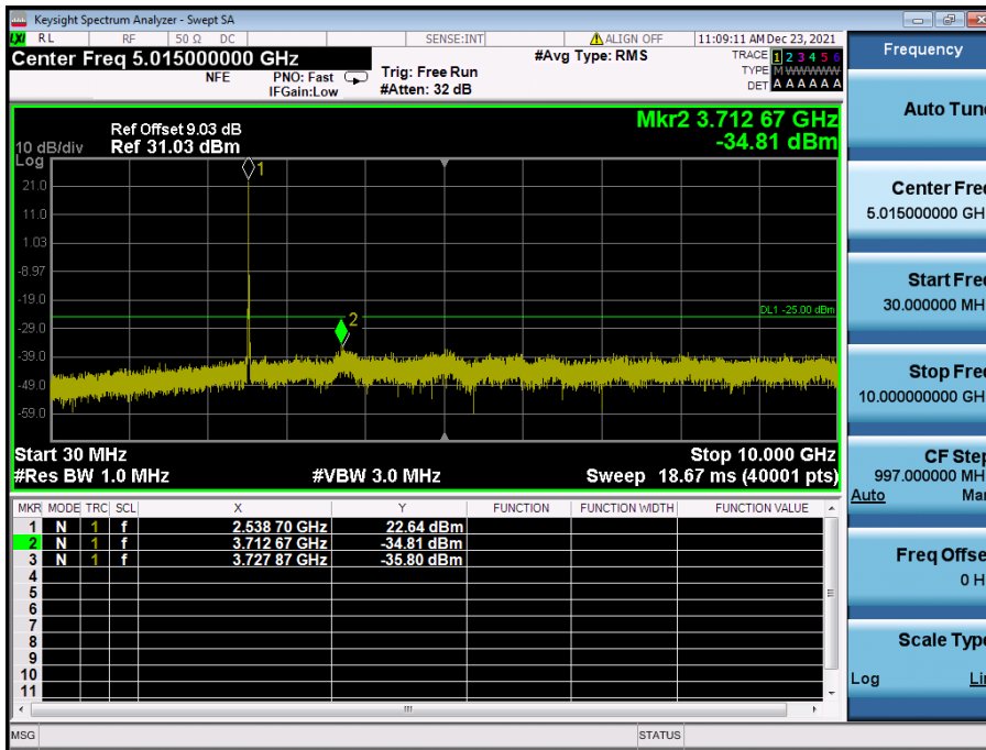
LTE Band 7 / 10 MHz / 16QAM - RB Size/Offset (25/25) – Mid Channel
