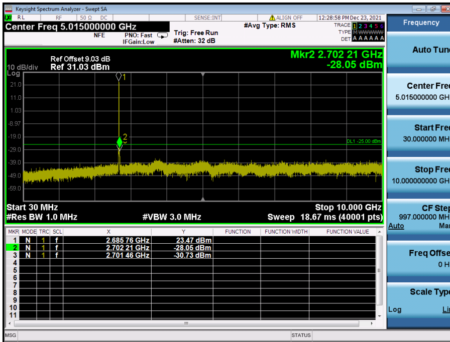
LTE Band 41 / 5 MHz / QPSK - RB Size/Offset (25/0) – High Channel
