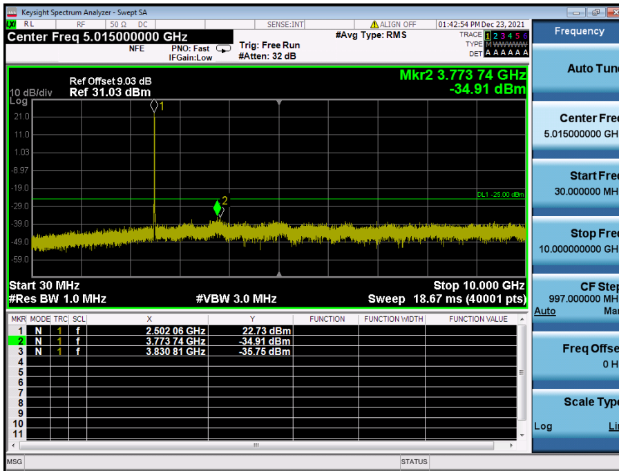
LTE Band 41 / 10 MHz / 16QAM - RB Size/Offset (25/25) – Low Channel
