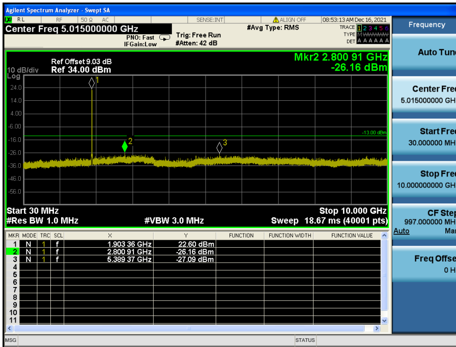
LTE Band 25(2) / 15 MHz / 16QAM - RB Size/Offset (36/0) – High Channel
