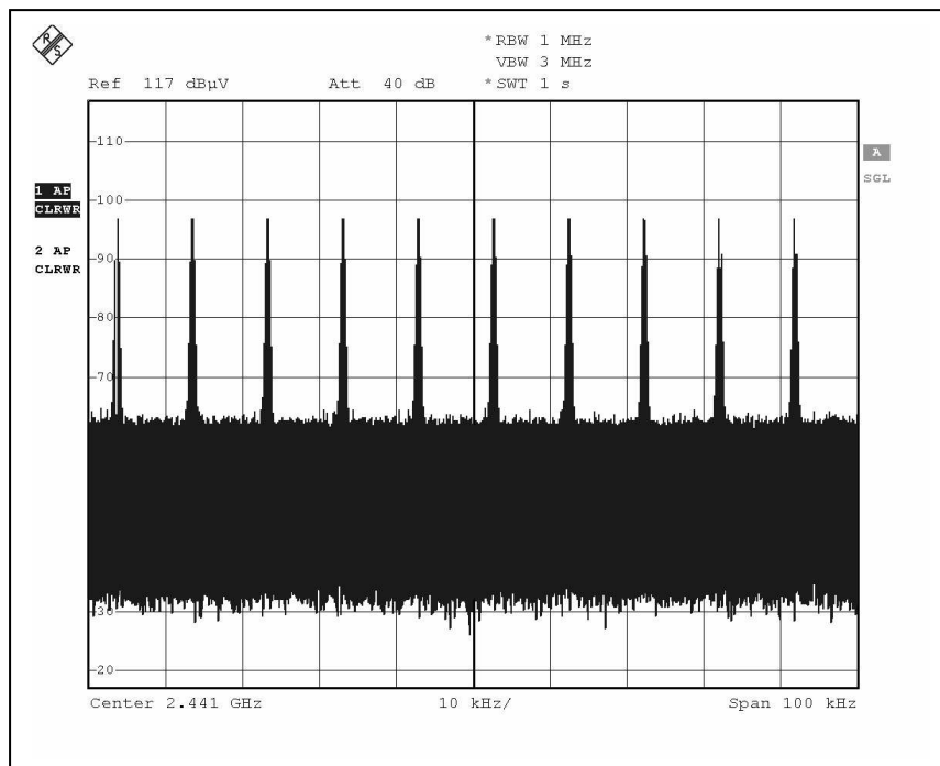
Transmitted carrier
