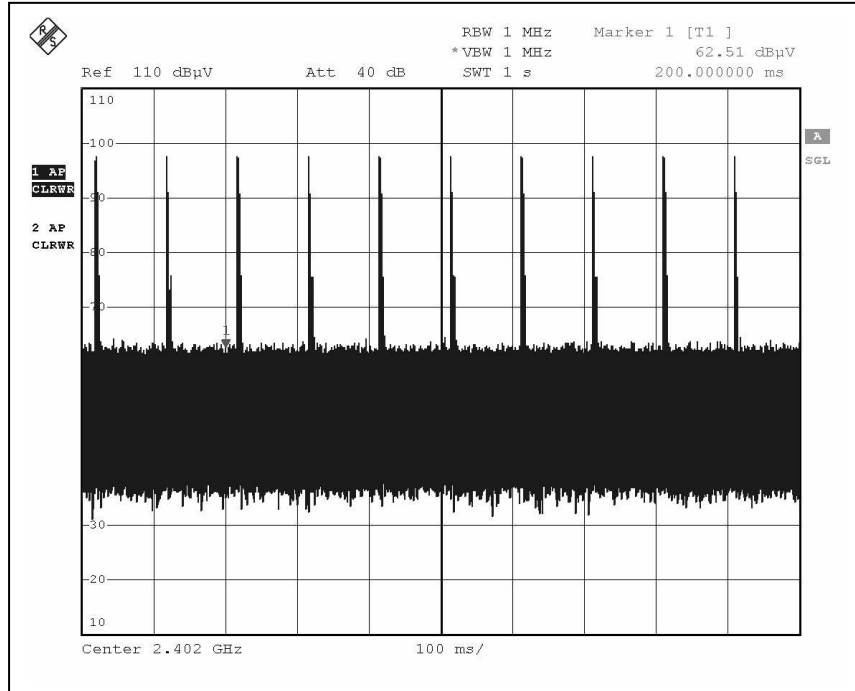
Transmitted carrier
