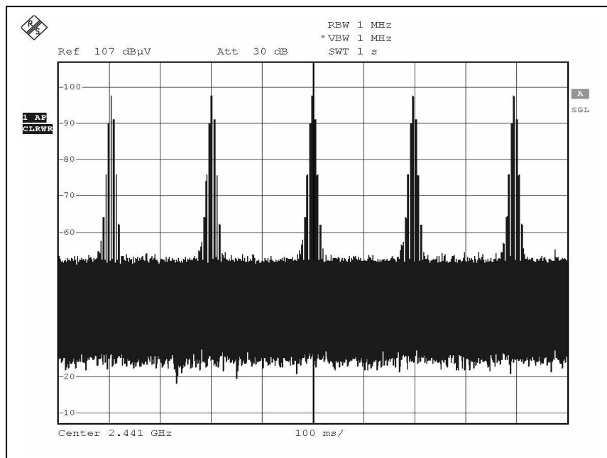
Transmitted carrier
