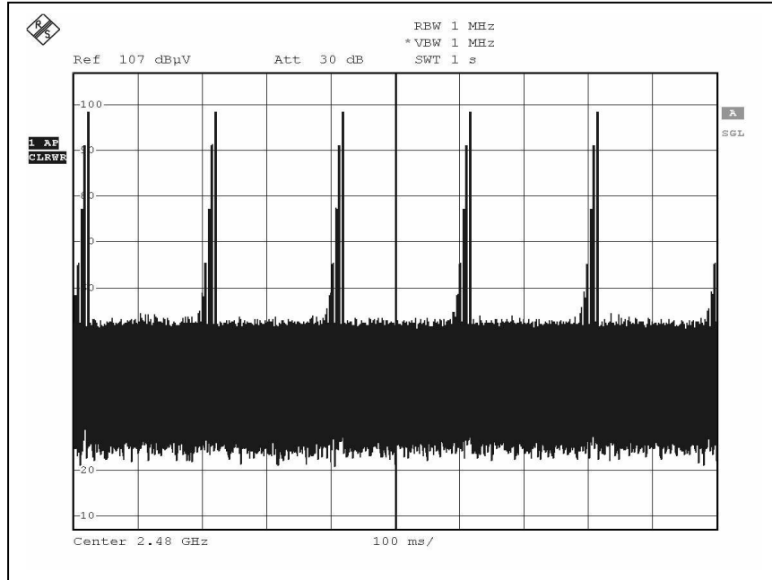
Transmitted carrier
