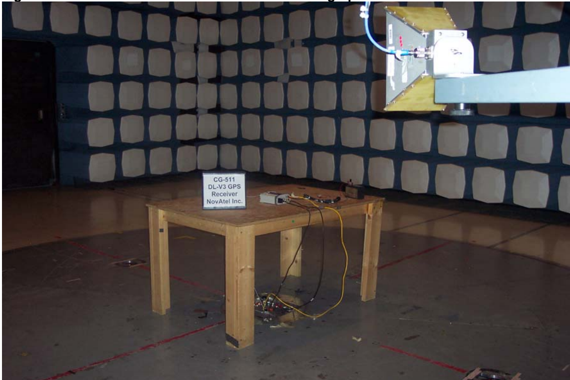
Figure 2 > 1 GHz Radiated Emissions Test Photograph
