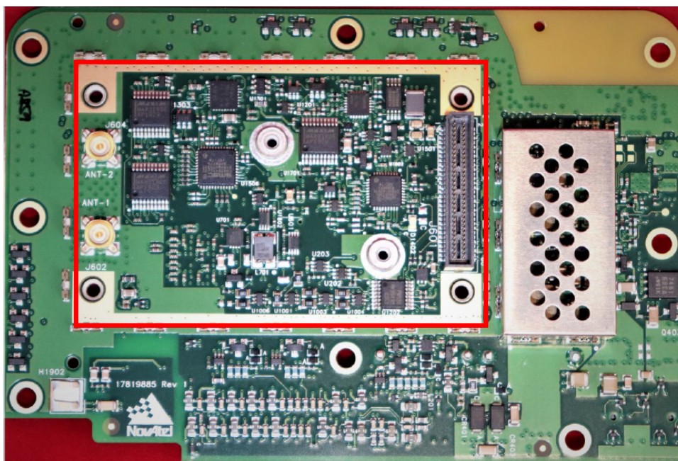
Figure 3 – PwrPak7D-E2 (01010282) Bottom PCB
