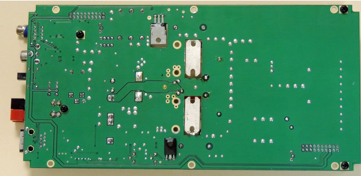
PA Board, Solder Side
