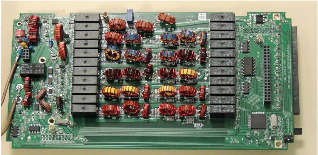
LPF Board, Component Side
