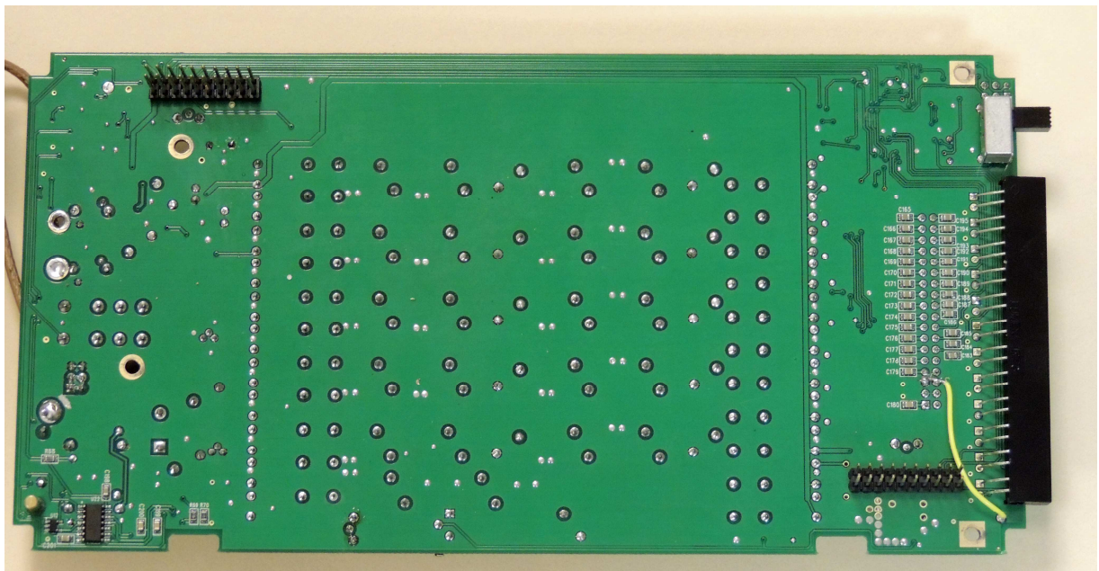
LPF Board, Solder Side
