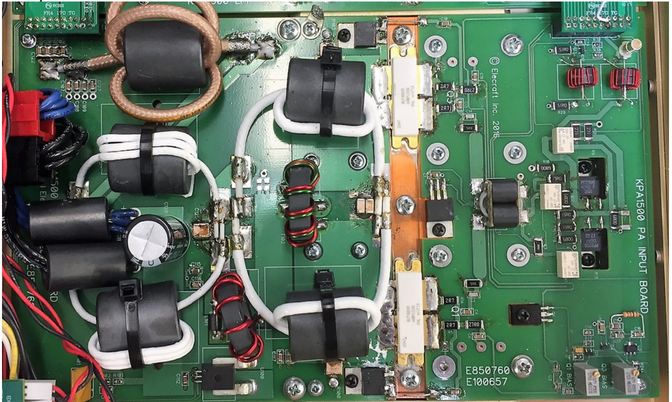
PA-top
