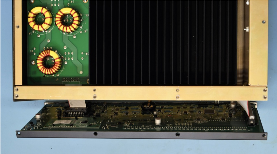
KPA1500 Top View Showing Front Panel Interconnection
