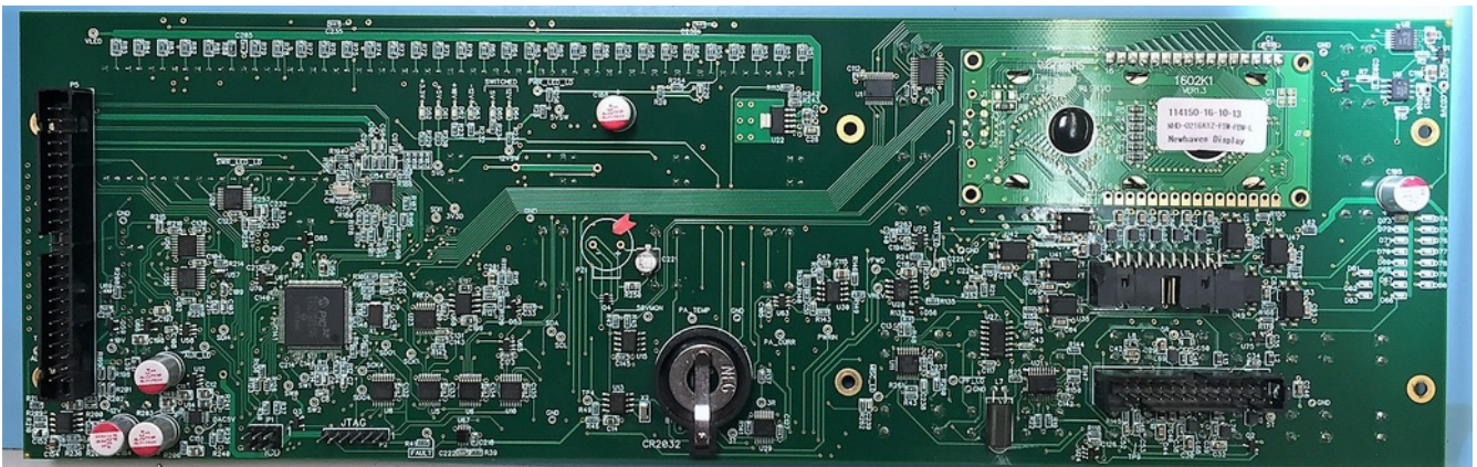
Front Panel-bottom
