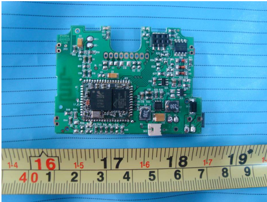
EUT – Main Unit Main Board Top View
