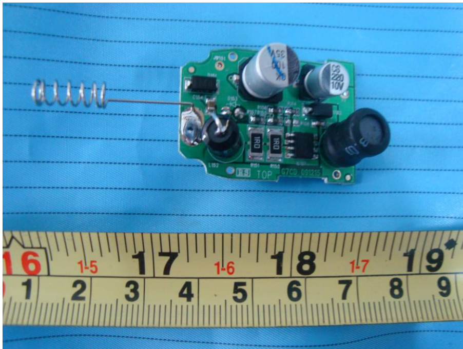
EUT – In-car Charger Main Board Top View
