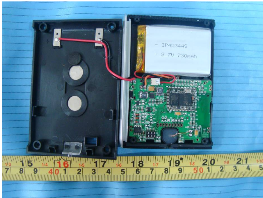
EUT – Main Unit Cover off View 1
