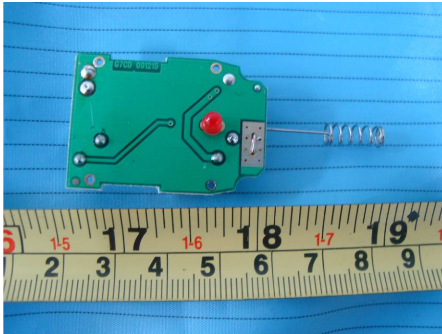
EUT – In-car Charger Main Board BottomView
