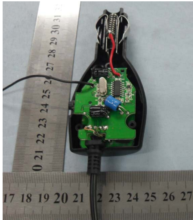
EUT- Uncoverd view
