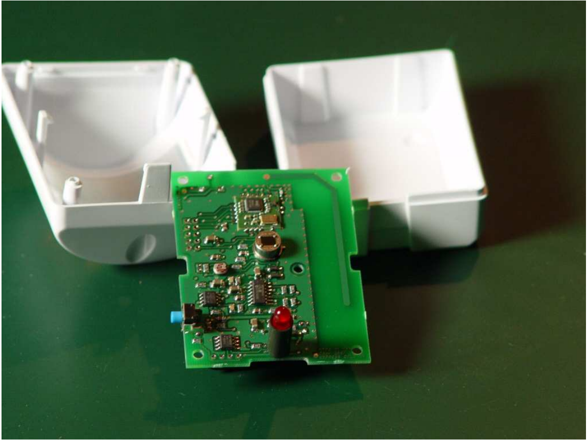
EZMotion Internal Photo – Component side
