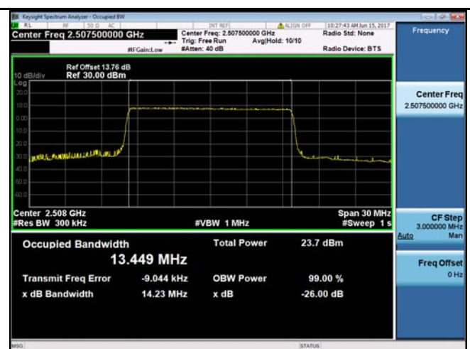
LTE band 7 - Low CH 16QAM-15
