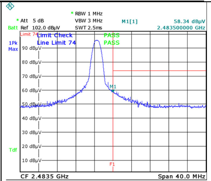
GFSK-Right Side-PK
