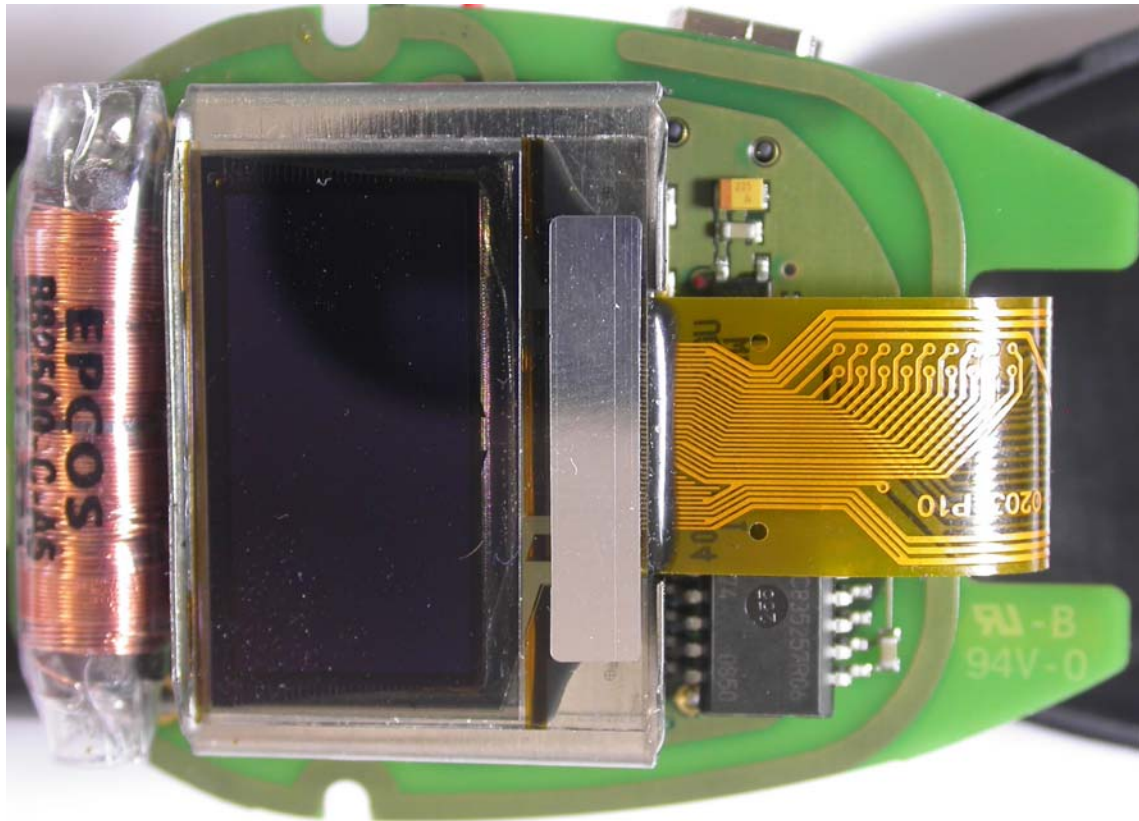
Front view PCB:
