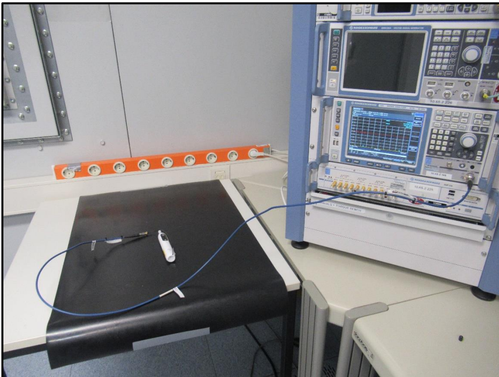
Photo 4 Conducted Test Setup
