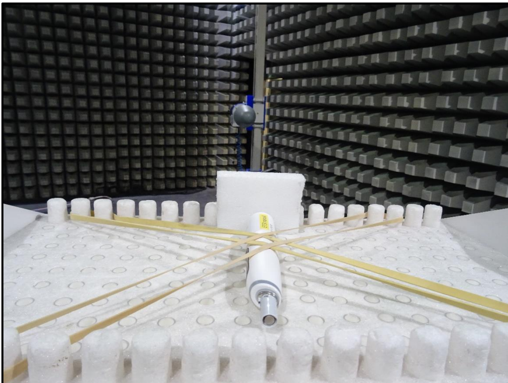
Photo 2 Radiated Test Setup ZX plane
