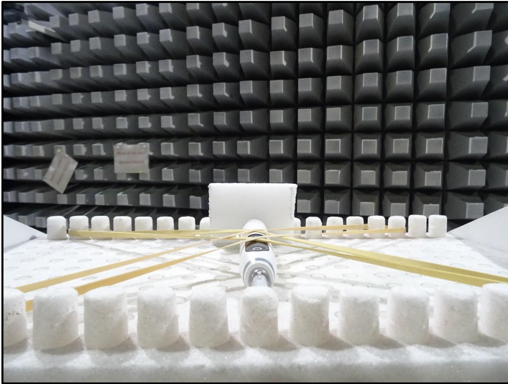
Photo 3 Radiated Test Setup YZ plane
