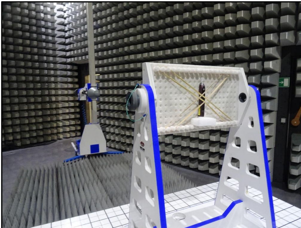
Photo 1 Radiated Test Setup XY plane
