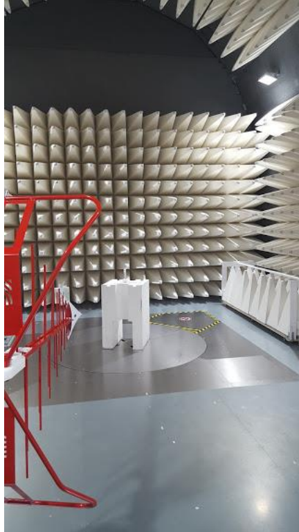
Figure B3. Radiated Emission Setup – Low Range
