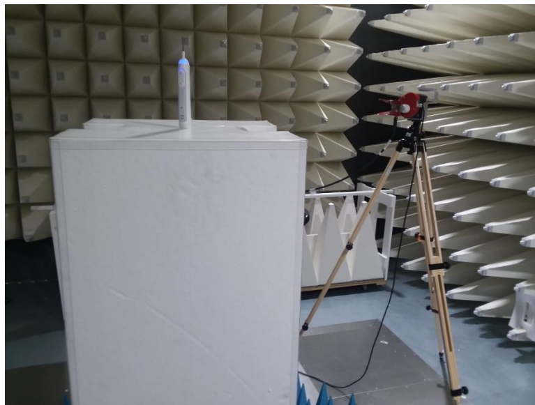
Figure B4. Radiated Emission Setup – High Range
