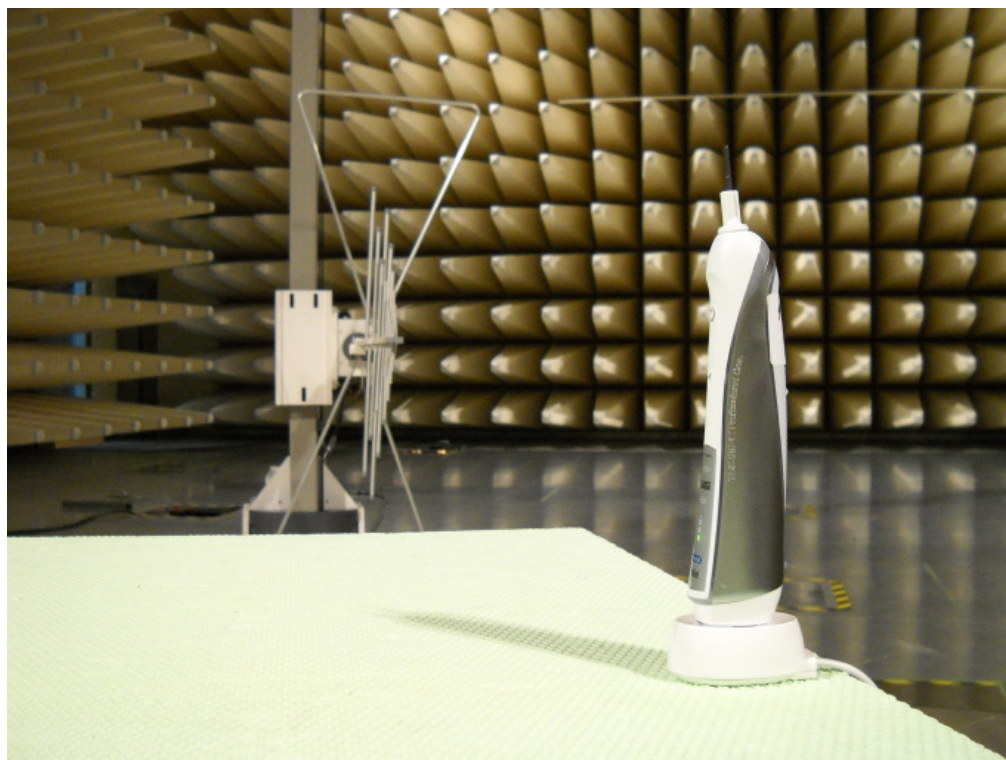
Figure 5 Radiated emissions, Charging
