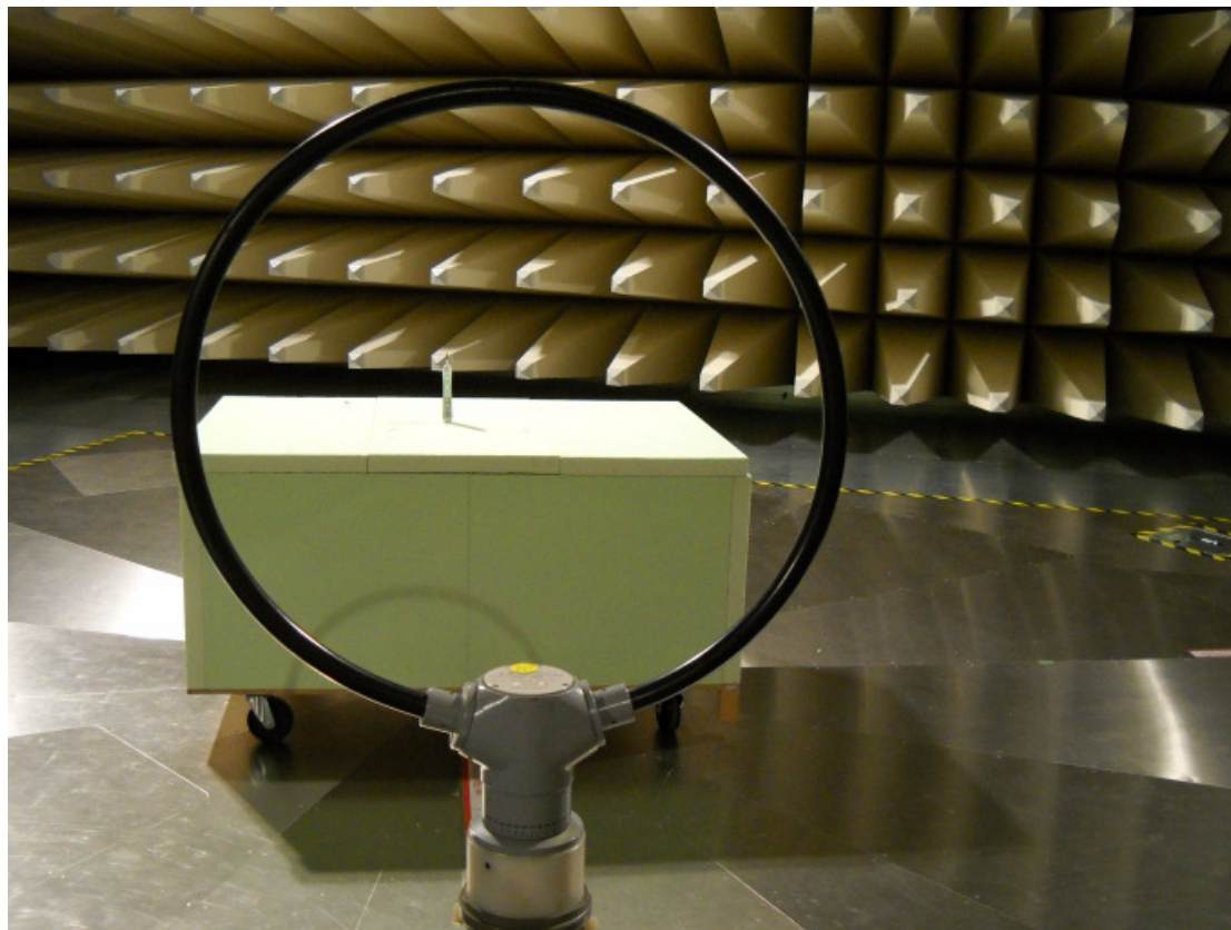
Figure 3 Radiated emissions in the frequency range from 9 kHz to 30 MHz (Brush mode)
