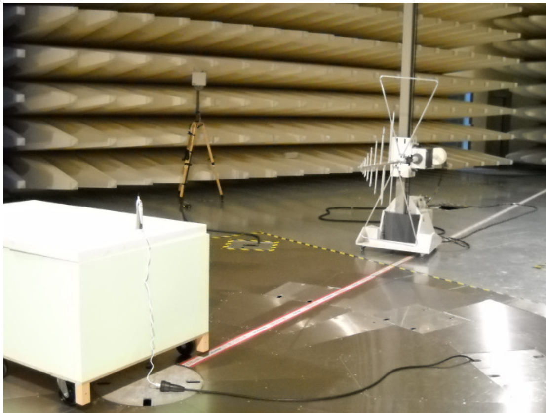
Figure 4 Radiated emissions, Charging
