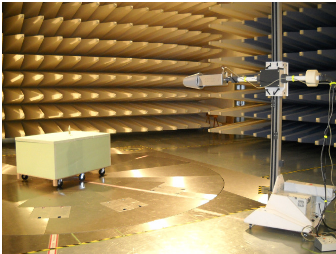
Figure 1 Radiated emissions at frequencies above 1 GHz (Brush mode, transmitter on)
