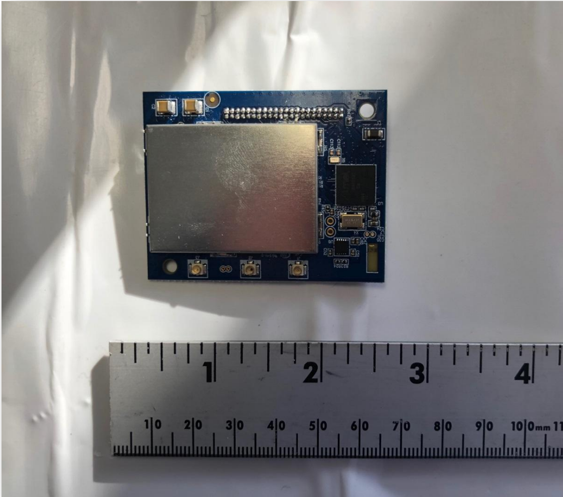
Figure 1. Top of EUT, with Shield
