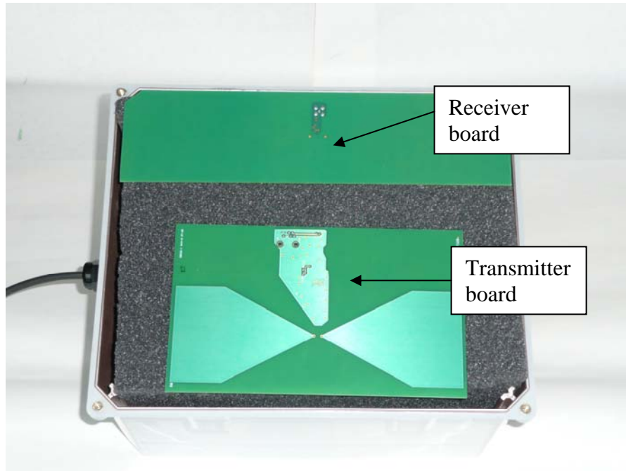
Cover removed, showing Receiver and Transmitter boards.
