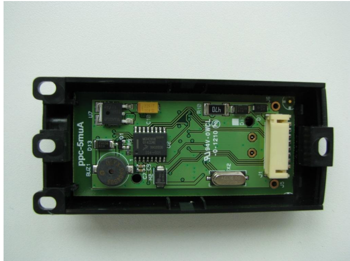
PCB in housing – unpotted
