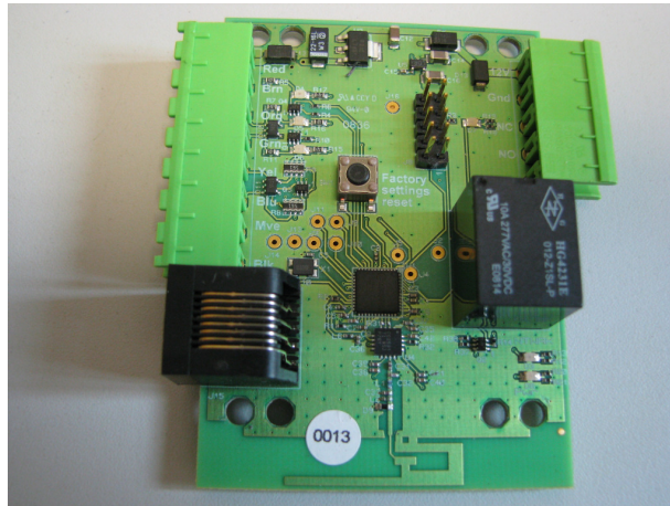
Wireless Reader Module PCB – top view
