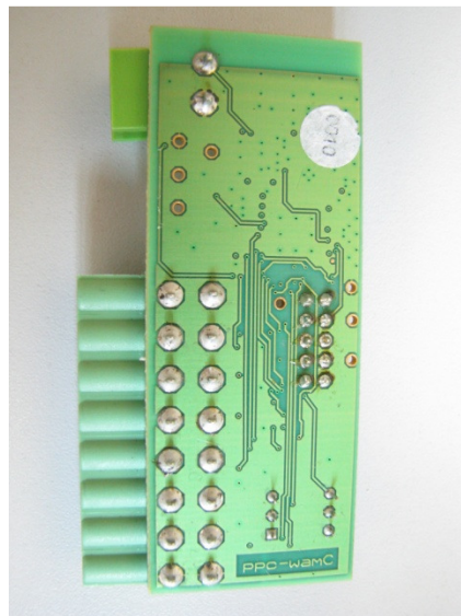
Wireless ACU Module PCB – back view
