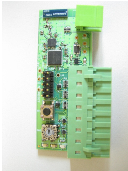
Wireless ACU Module PCB – top view
