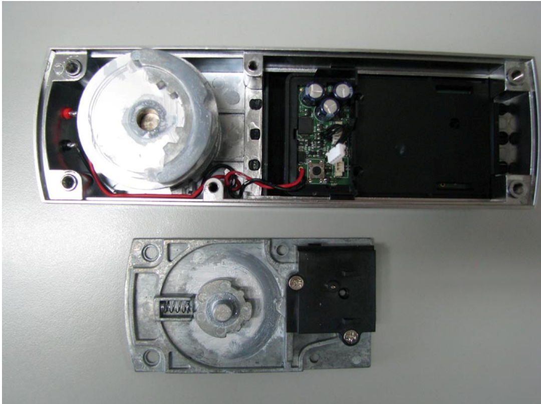
PCB and coil former inside metal housing with lock assembly
