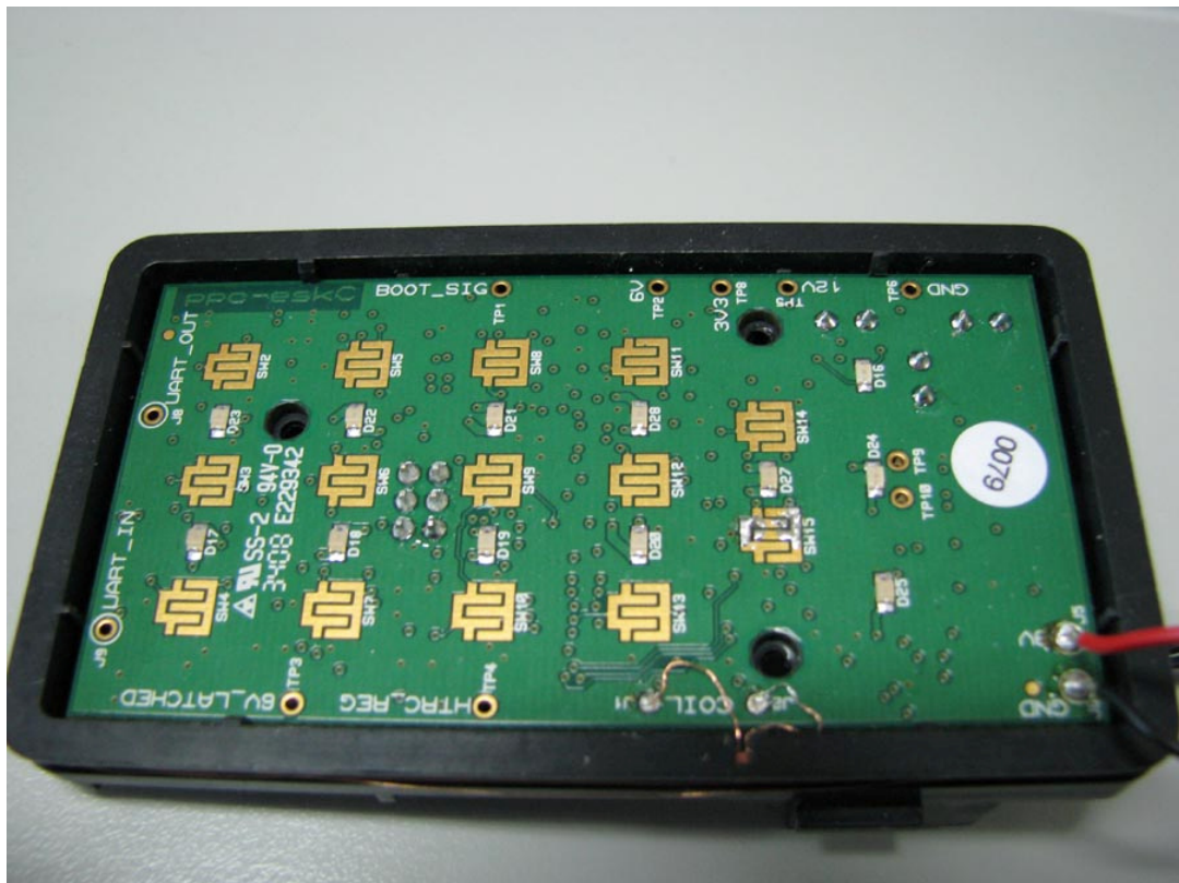
Main PCB (front) located inside plastic coil former (antenna)
