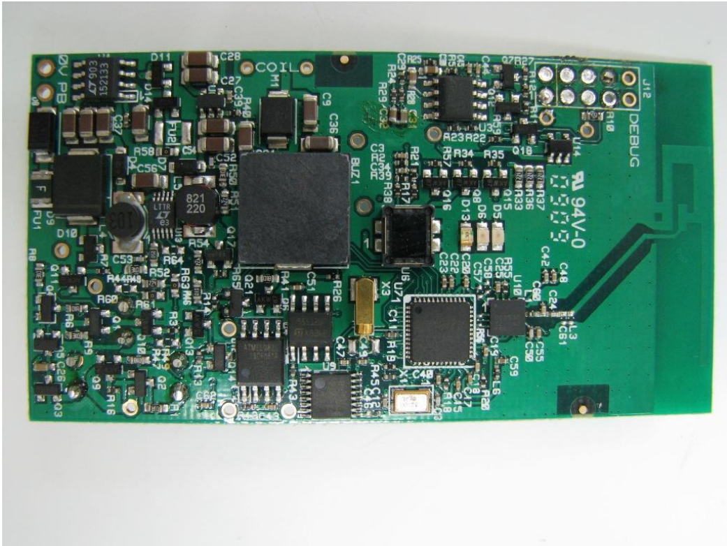
Main PCB Front
