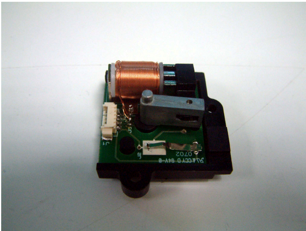
Bistable latch mechanism and switch pcb
