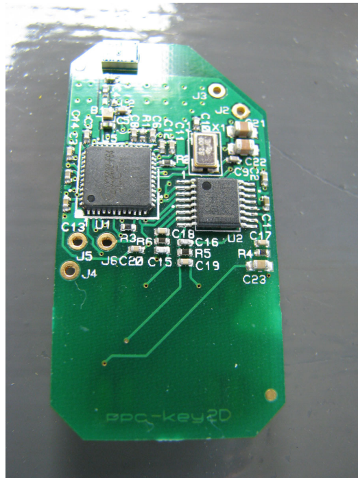
PCB - top view
