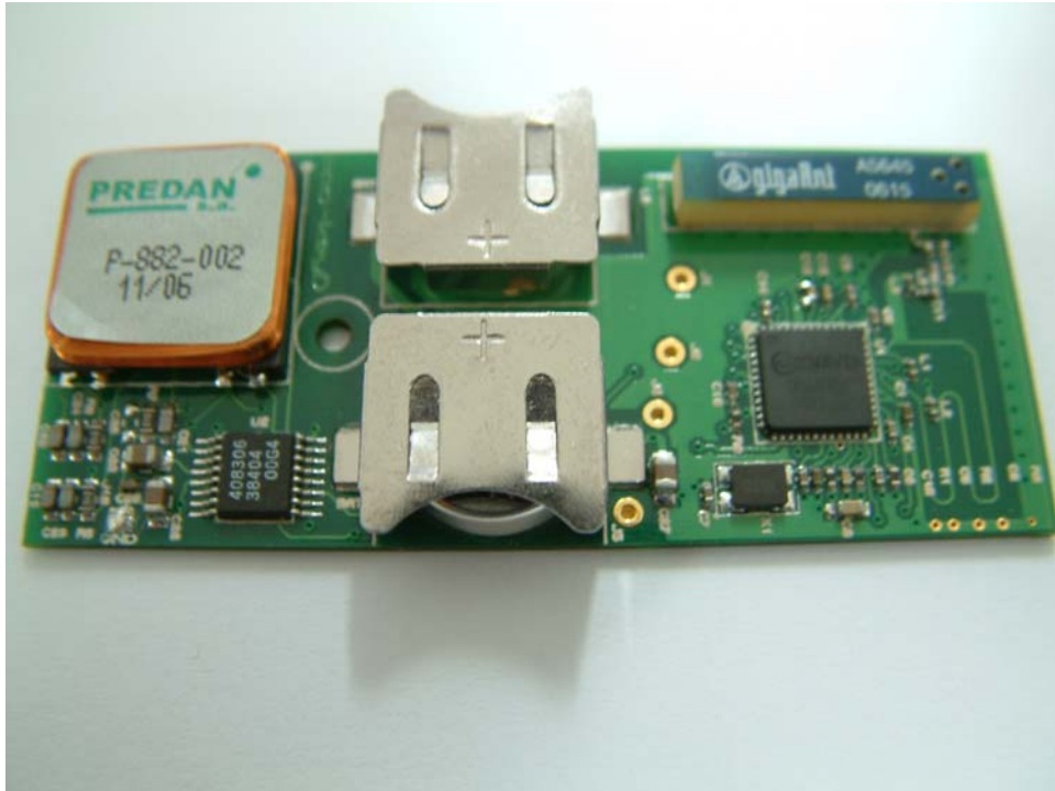
Keyfob PCB Top View
