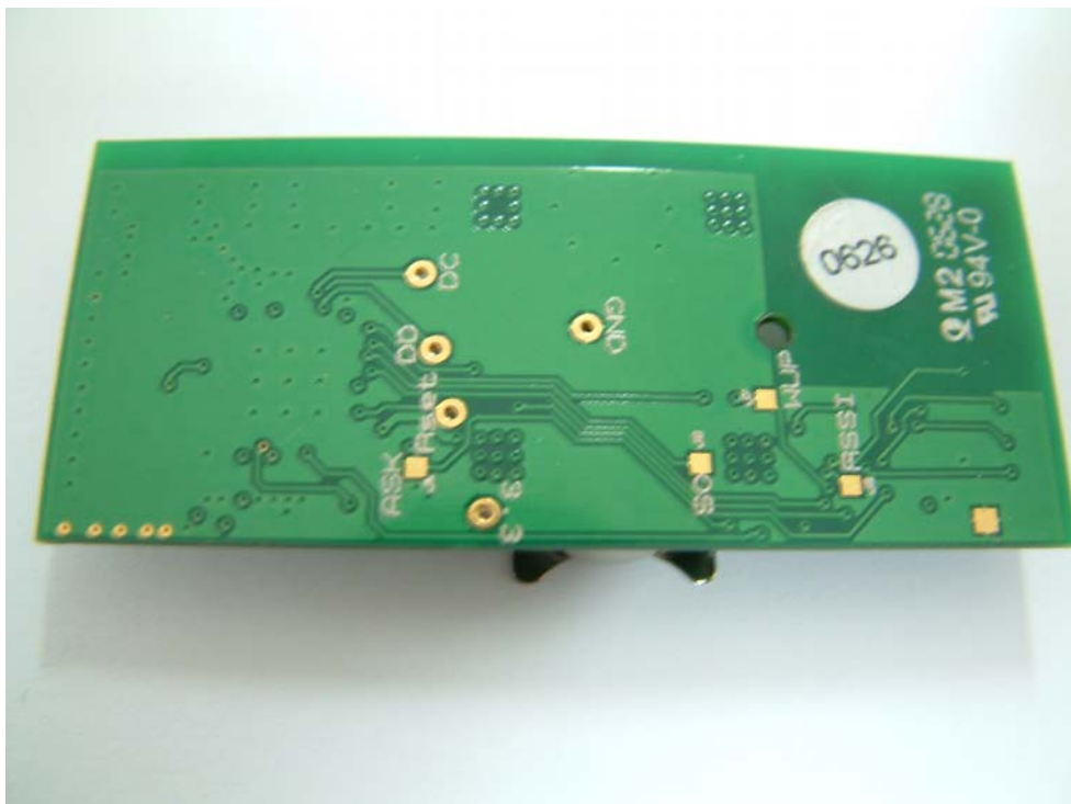
Keyfob PCB Bottom View
