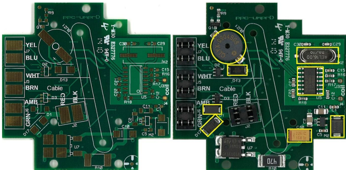
Unpopulated PCB
