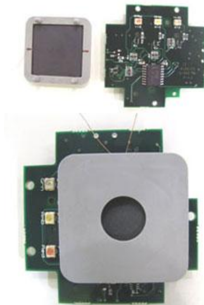
Antenna/coil former attachment to circuit board.
