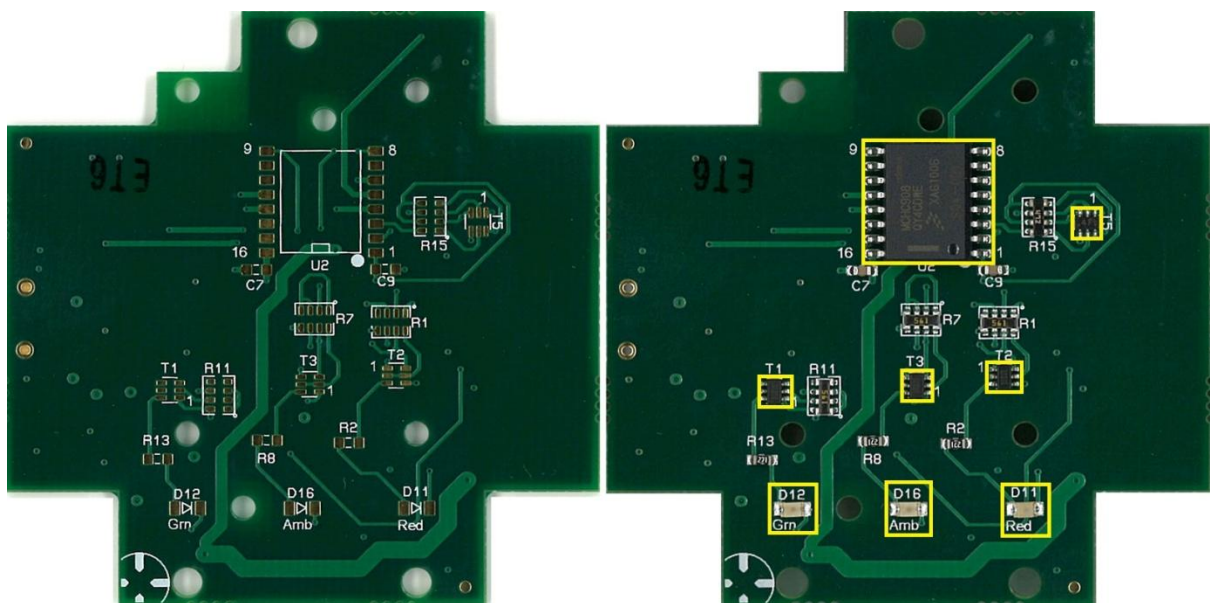
Unpopulated PCB
