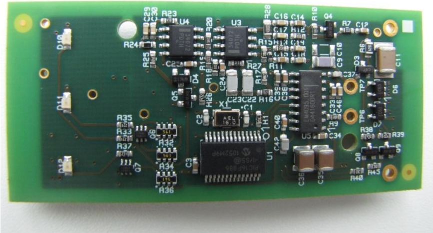
PCB top view
