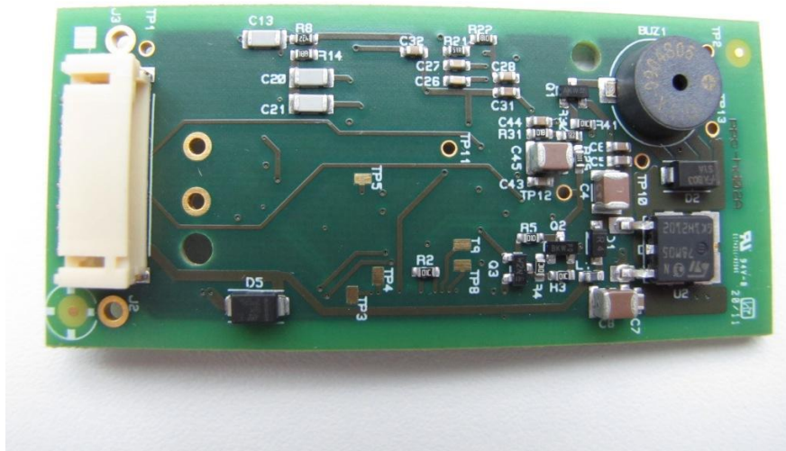
PCB bottom view
