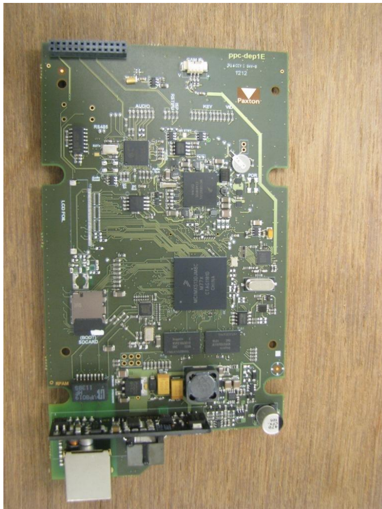
Main Panel CPU board – top view
