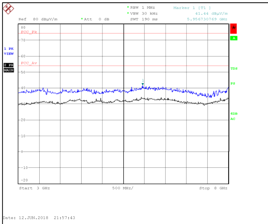
Figure 5 - 3 GHz to 8 GHz - Horizontal and Vertical
