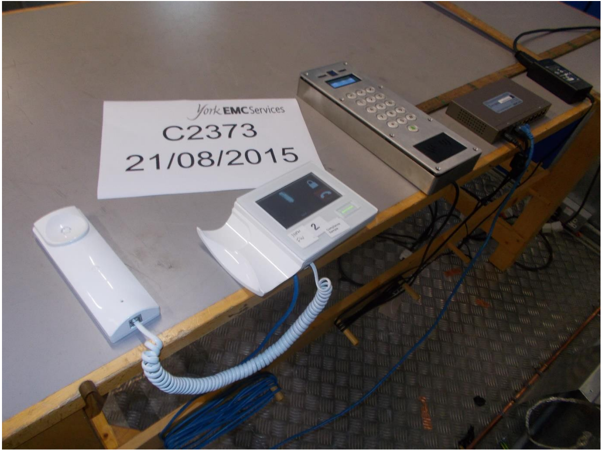
Conducted emissions
