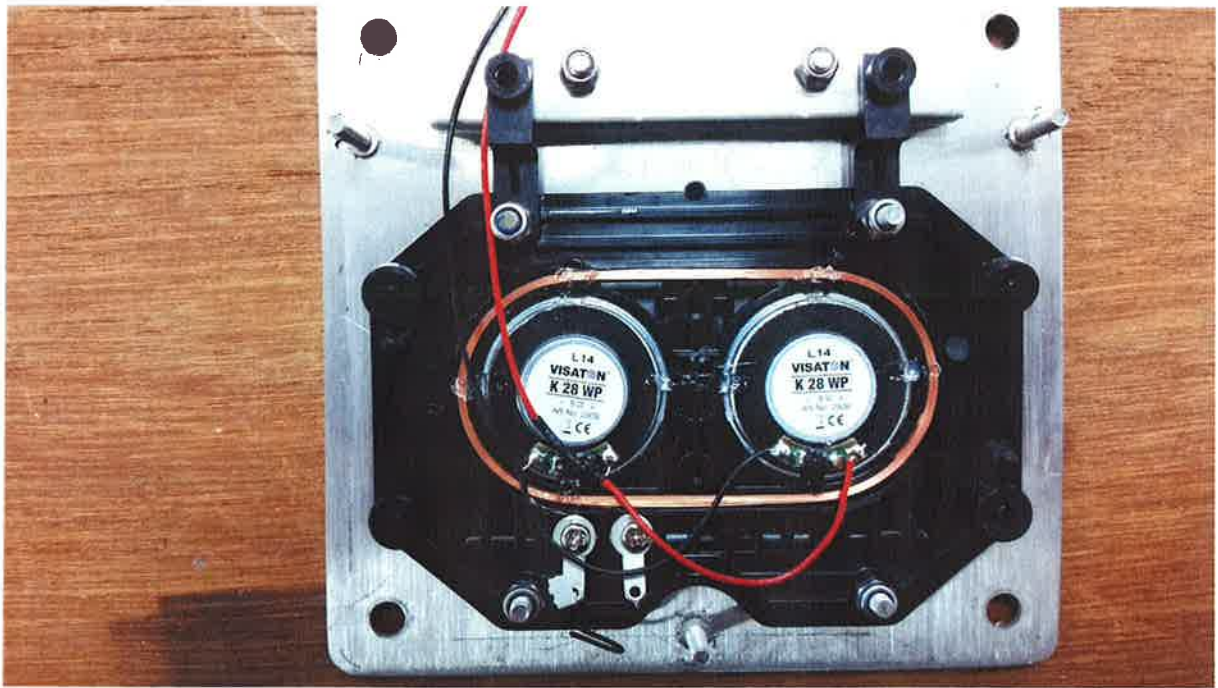
Figure 10 - Reader Rear
