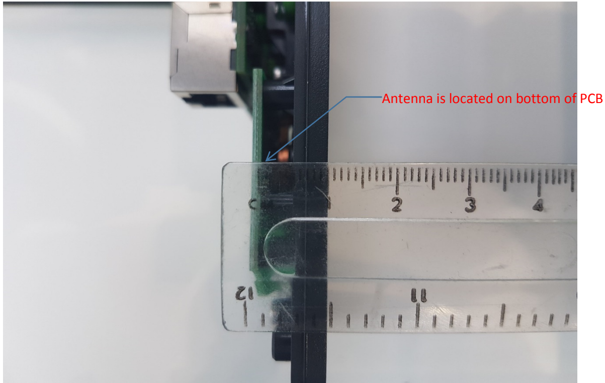
Shortest distance from the Antenna to the case – this is to the edge of the front panel and is 10mm
