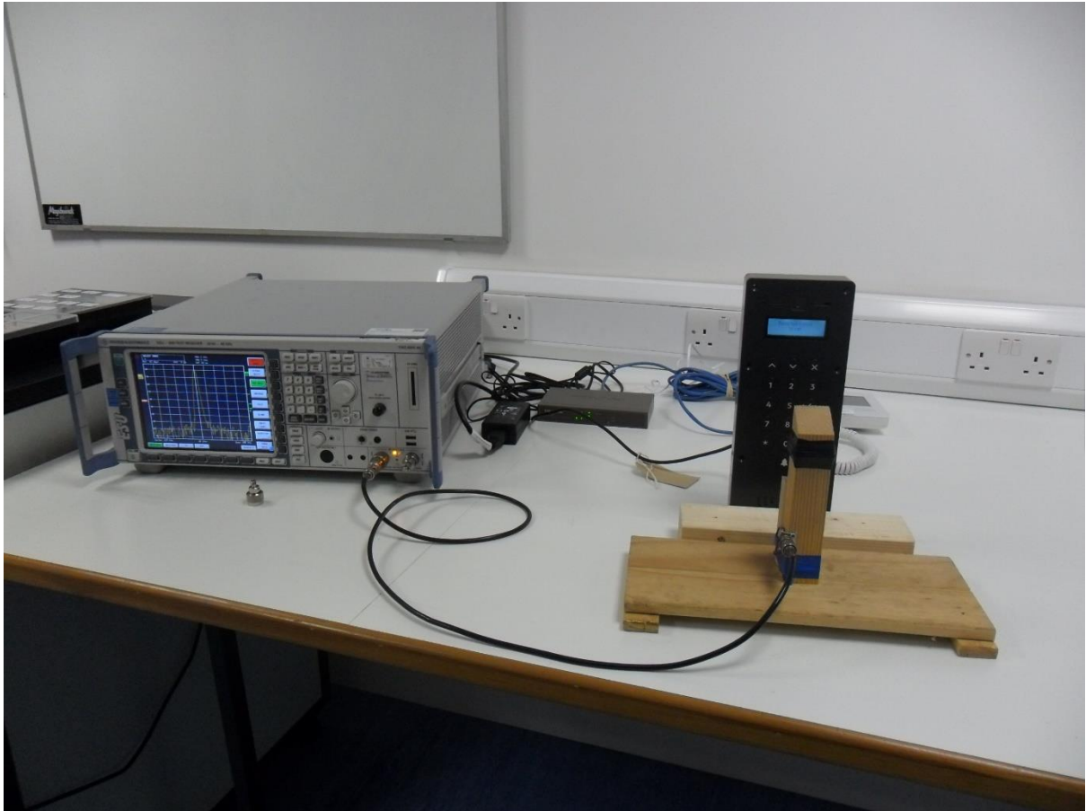
Frequency Tolerance Test – Standard Model
