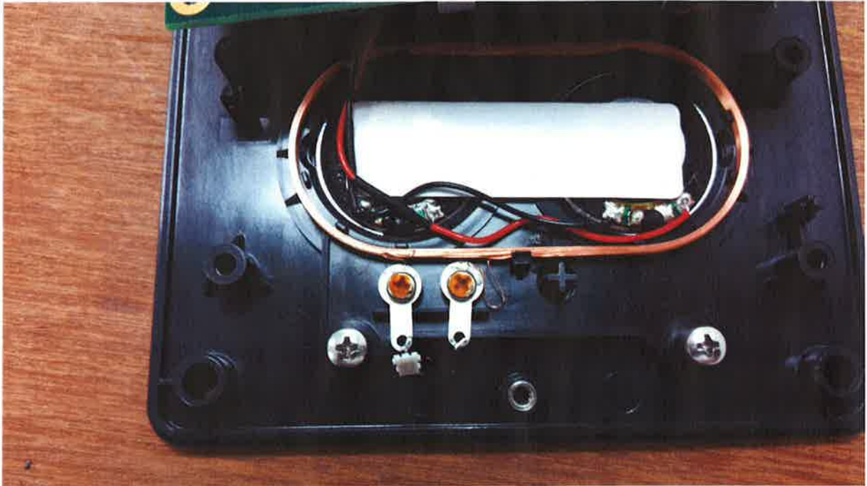
Figure 10 - Reader Rear
