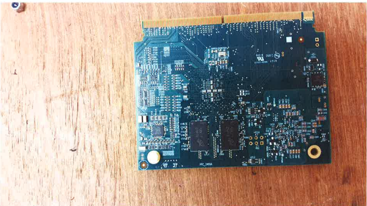
Figure 3 - Daughter card rear
