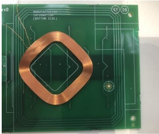
Photo 1. Front PCB Bottom, showing both antennas
