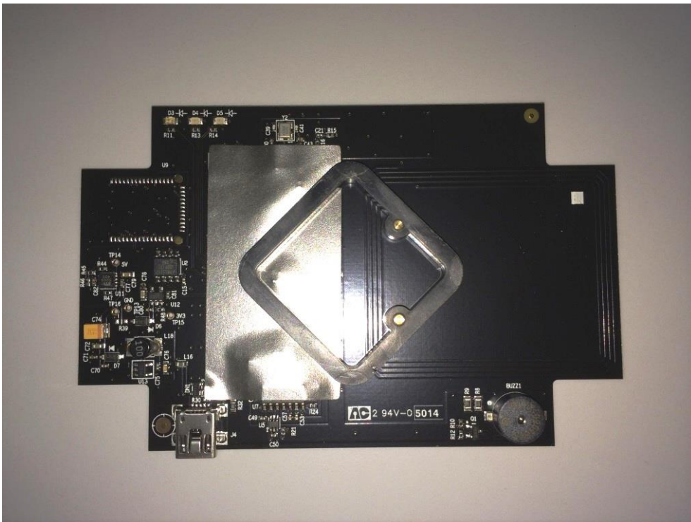
PHOTO 2 – PCB top view
