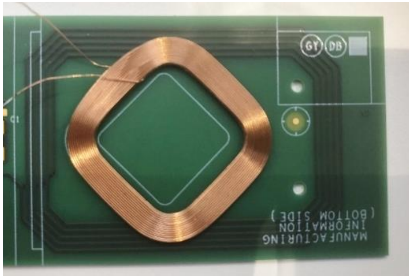
Photo 1. Front PCB Bottom, showing both antennas
