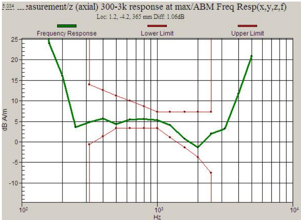
Graph 2 : CDMA 800 (CH 384) Frequency Response
