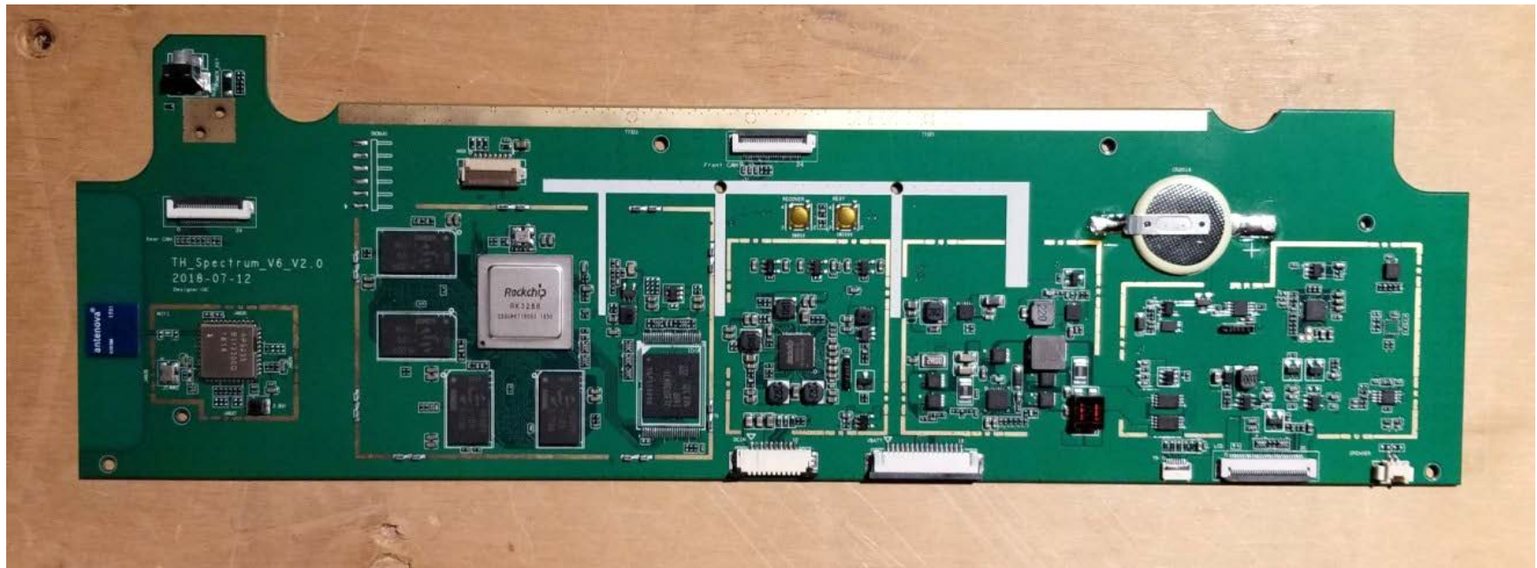
Photograph 16 – 2400-00429 main CPU assembly top side and bottom side
