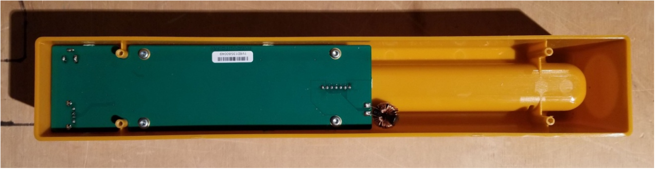
Photograph 25 - USB docking cradle bottom view with bottom removed
