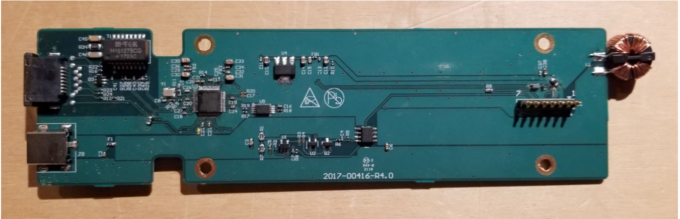
Photograph 23 - 2400-00427-R6 Ethernet docking cradle circuit board top side
