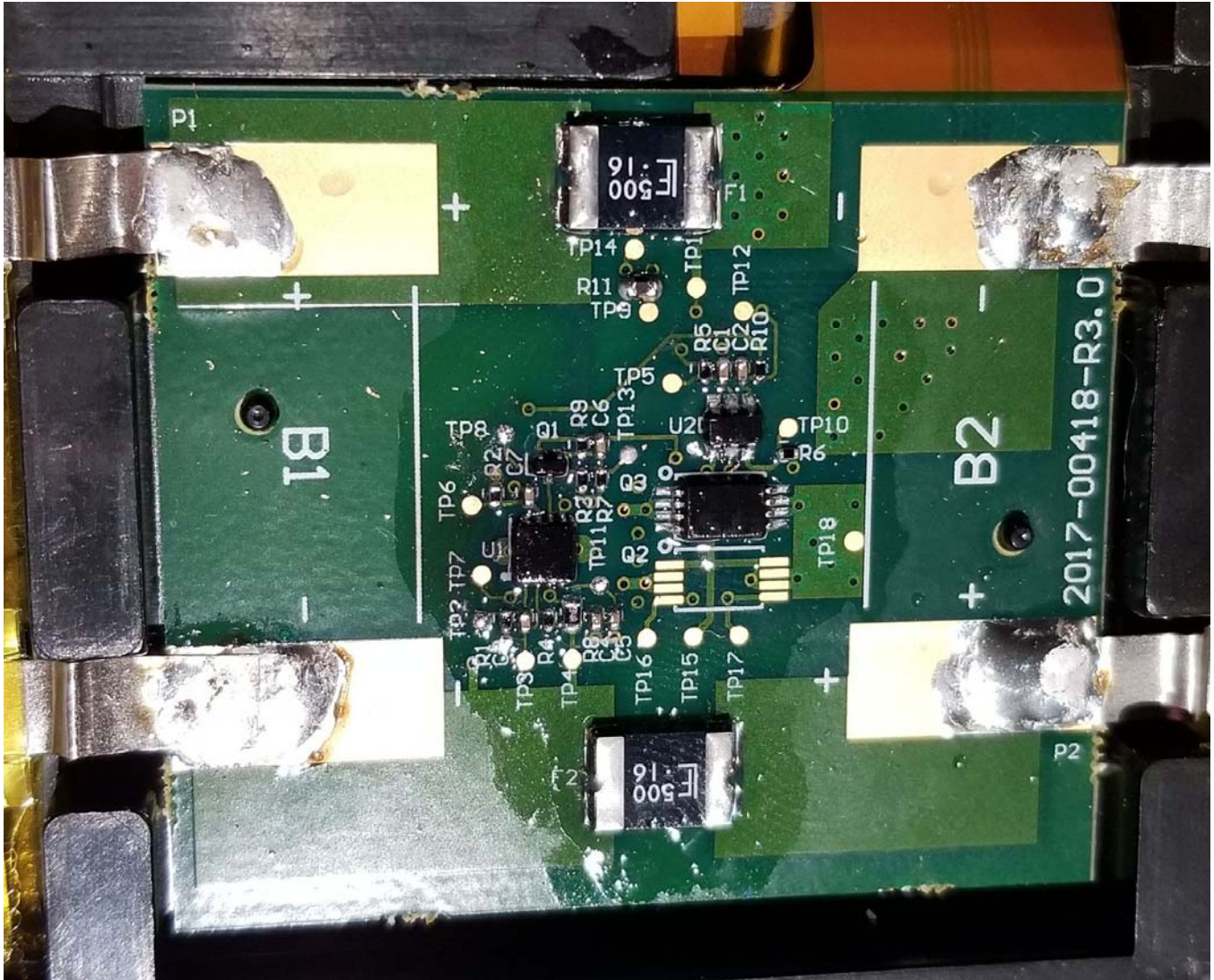
Photograph 28 – 2400-00428 Circuit detail
