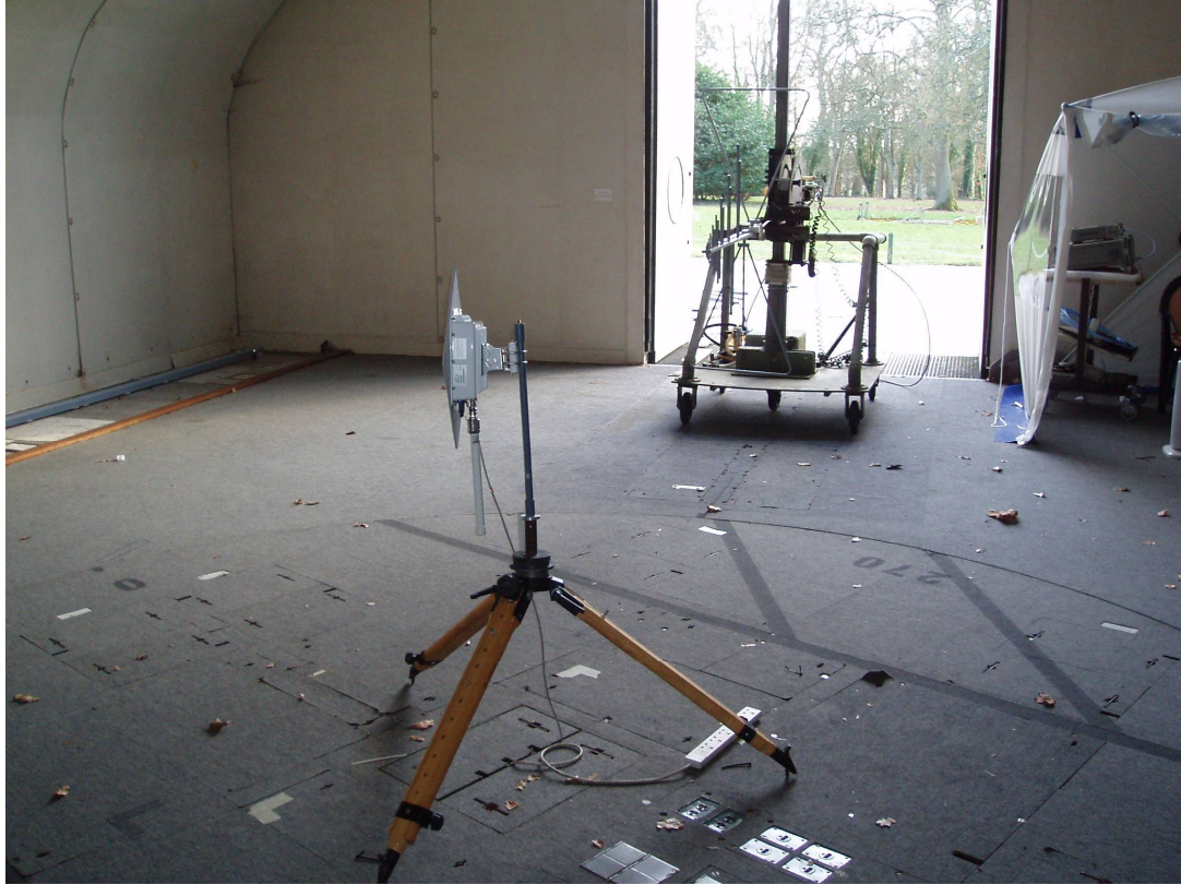
Hursley EMC OATS test site: measurements < 1GHz
