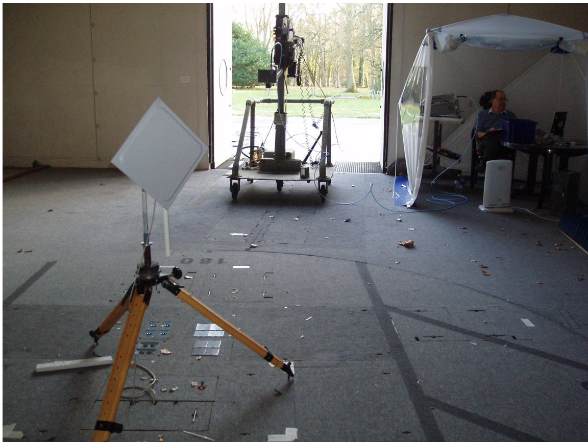
Hursley EMC OATS test site: measurements > 1GHz
