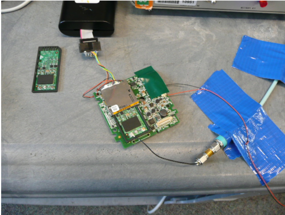
Figure 5 – Conducted Measurements Close up
