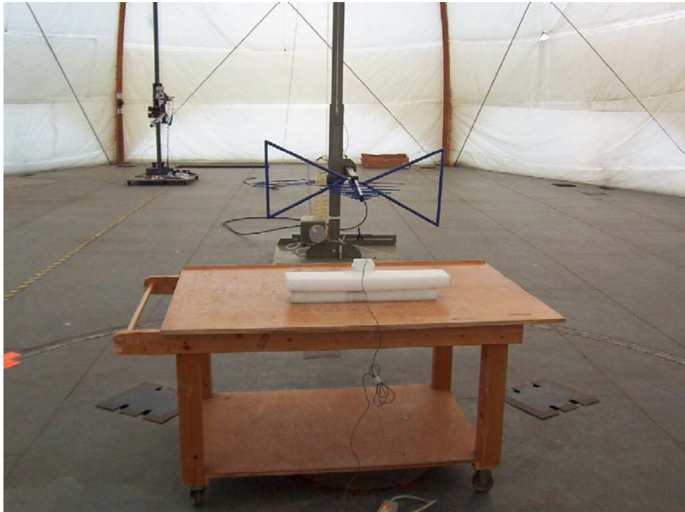
Figure 2 – Finals at OATS
