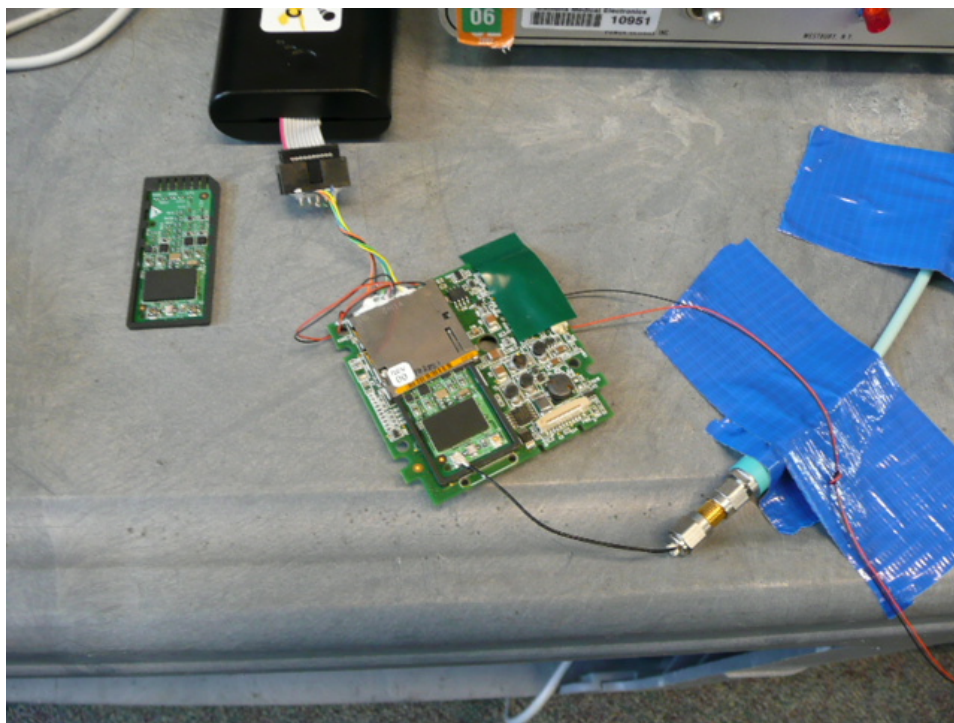
Figure 5 – Radio as tested on the bench
