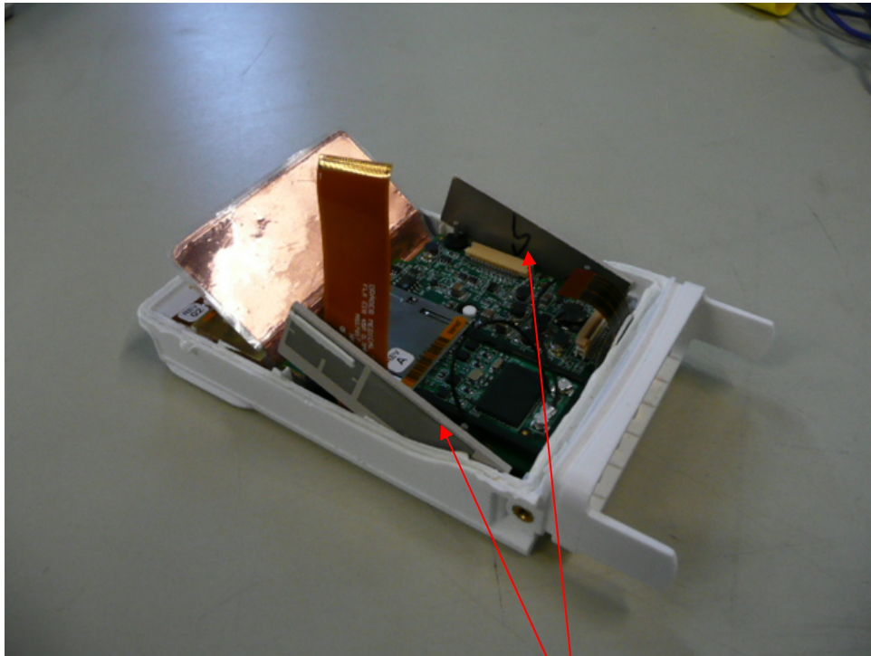
Figure 2 – Antenna's in M300
