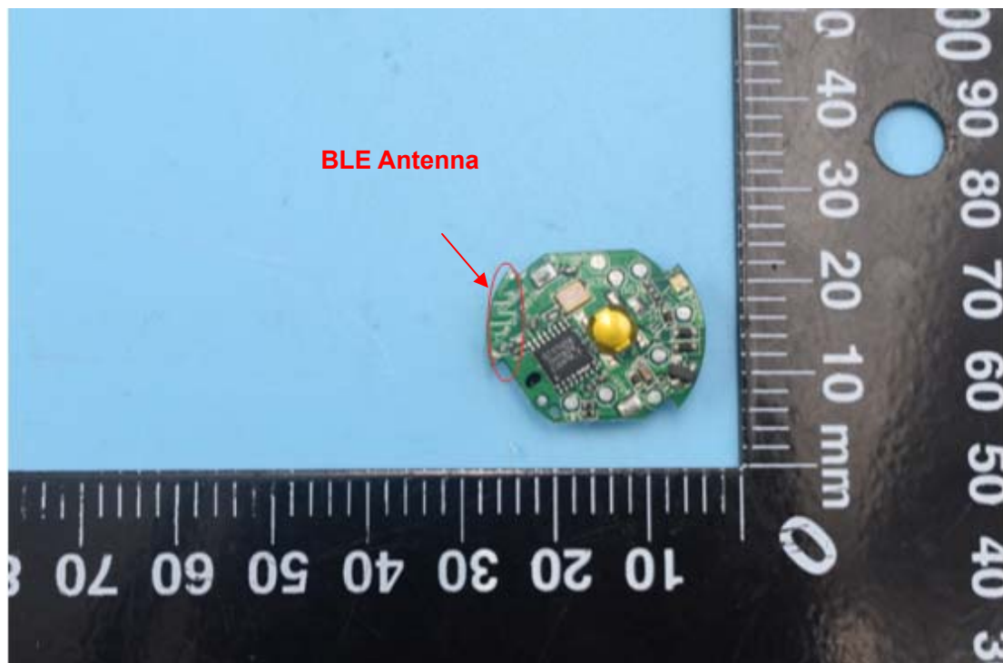
2. Antenna view
