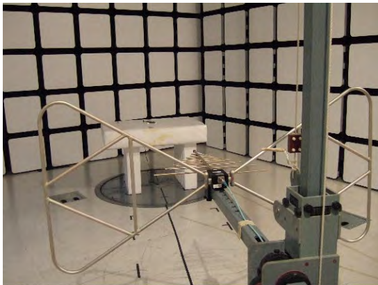
Test Configuration 2: 30 MHz to 960 MHz
