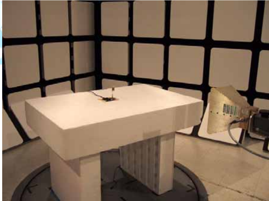
Test Configuration 3: 960 MHz to 40 GHz
